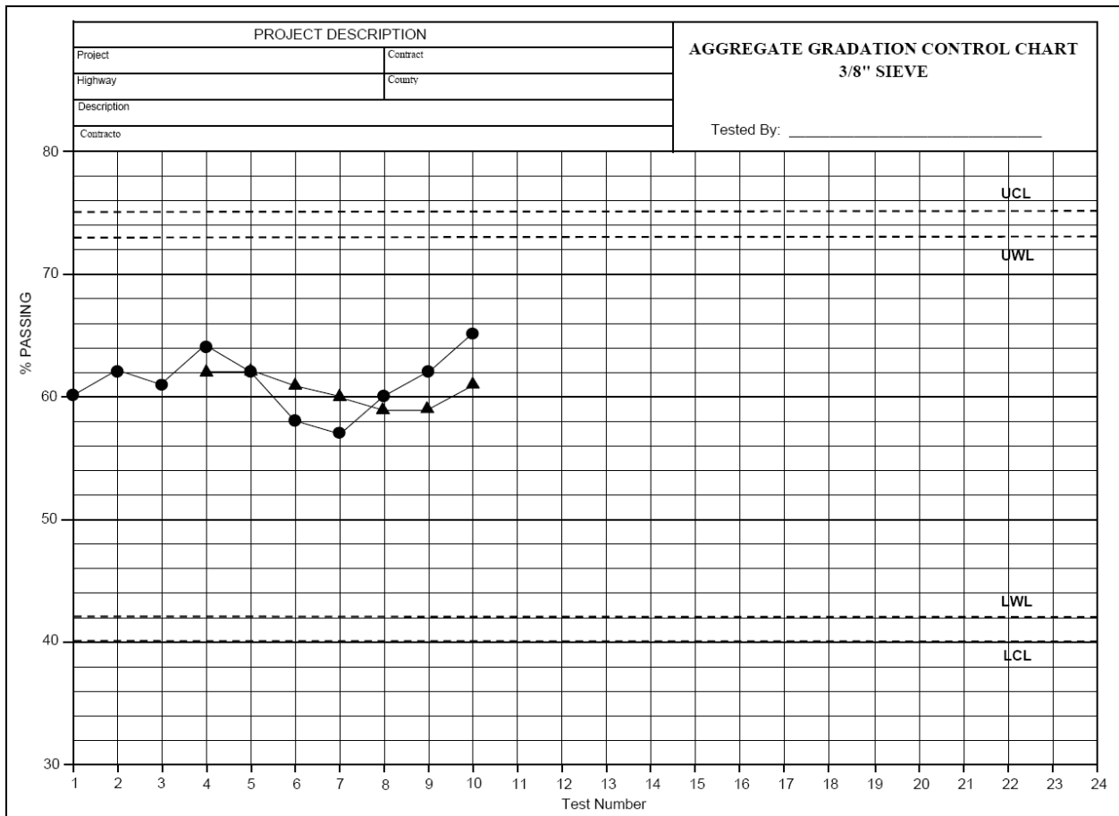
Figure 4: Example Aggregate Gradation Control Chart, 3/8" Sieve, Form WS3017
